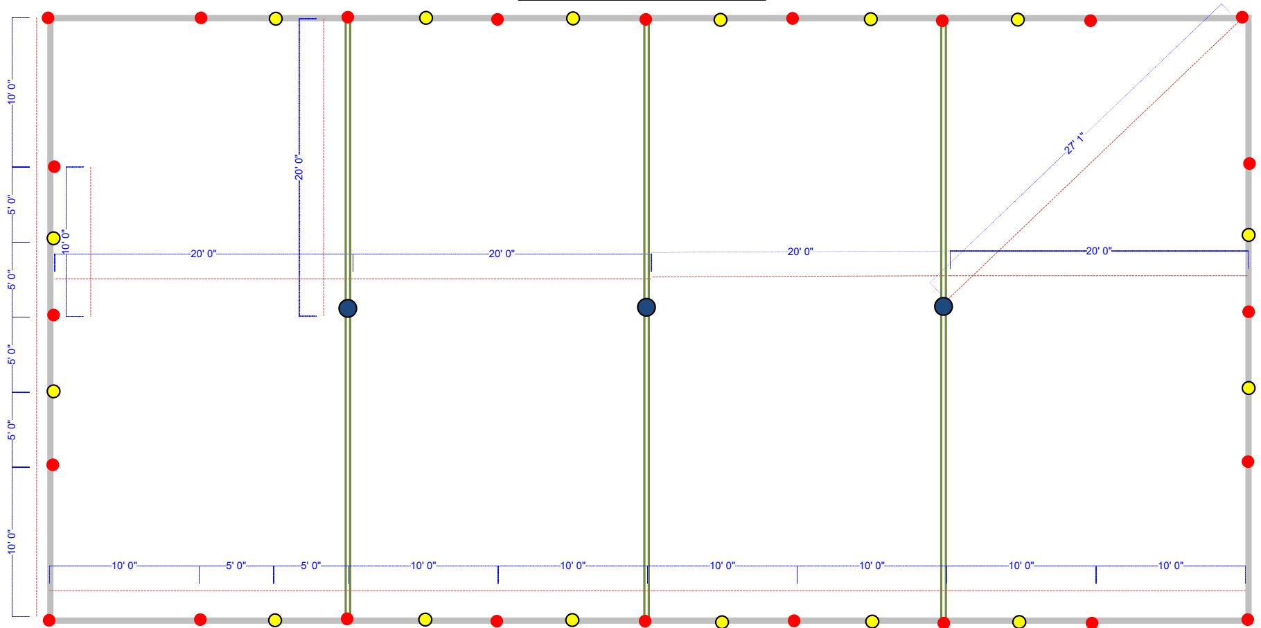
40' x 80' Pole Tent Standard & Wind - Pole Placements
